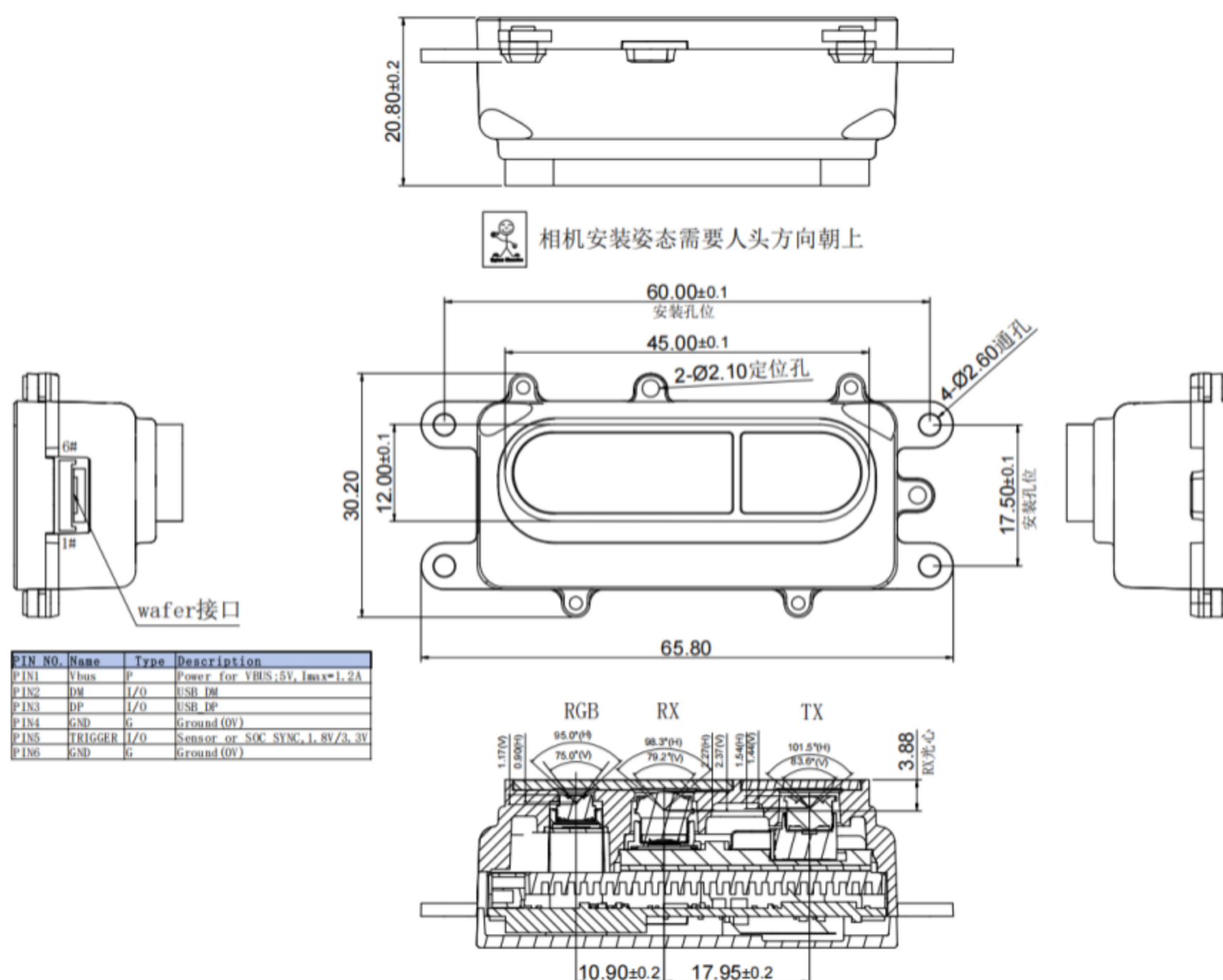
Module dimension drawing (65.80 mm × 30.20 mm × 20.80 mm, incl. mounting holes, wafer connector, and FOV annotation)
