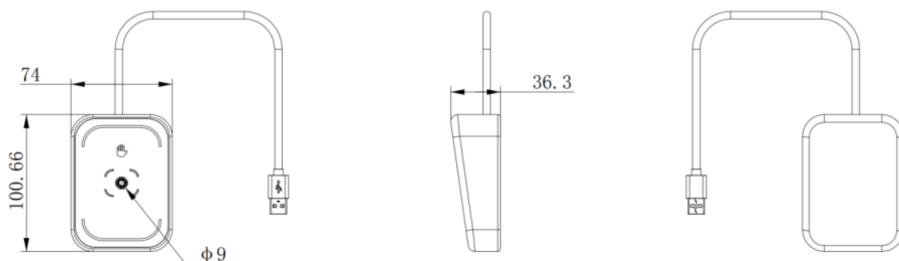
Dimension drawing
