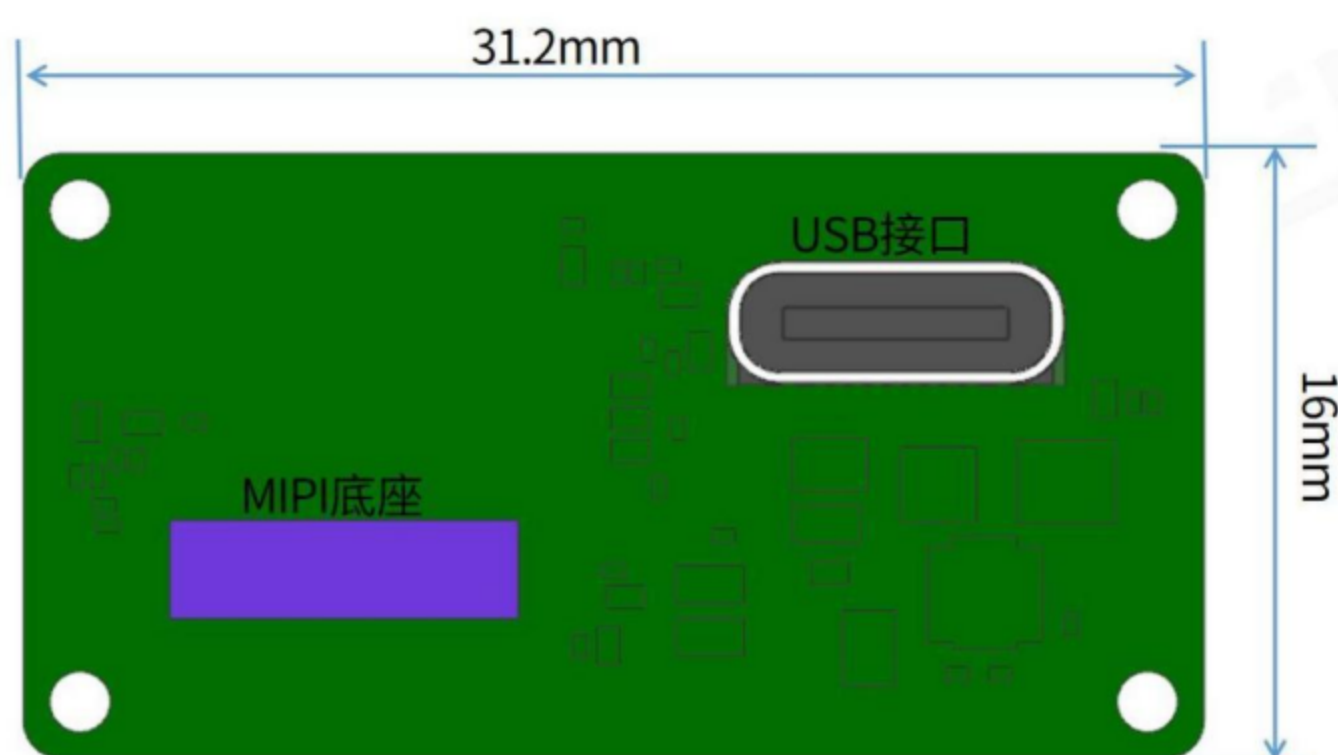
PCBA dimension drawing (31.2 mm × 16 mm, incl. USB connector and MIPI socket)
