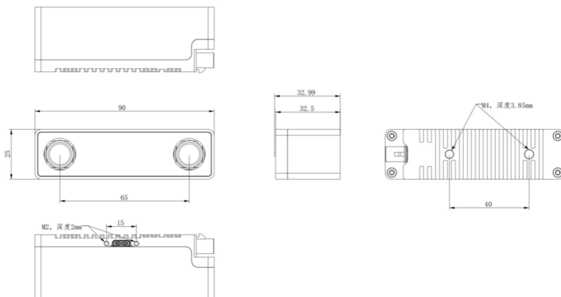
Figure: Module dimension drawing (90 × 25 × 32.99 mm)
