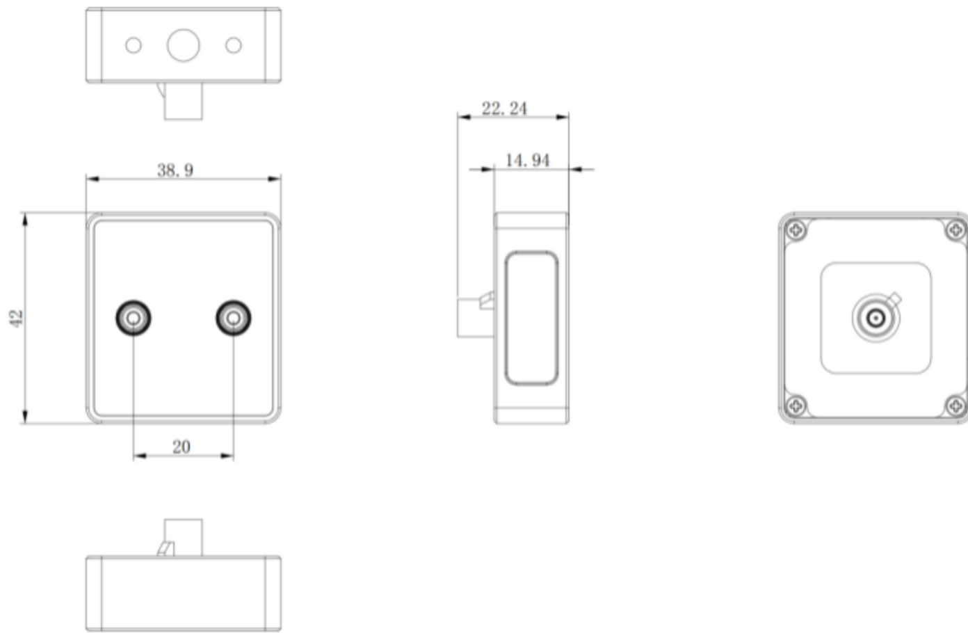
Module dimension drawing ( 38.9 \times 42 \times 22.24 mm)
