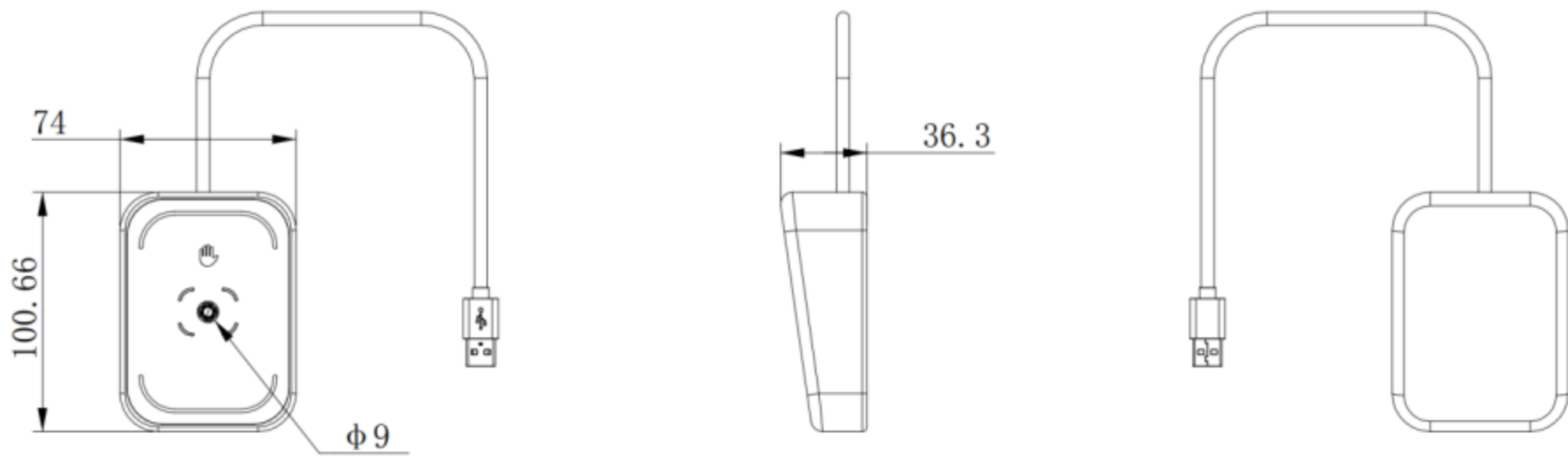
Dimension drawing
