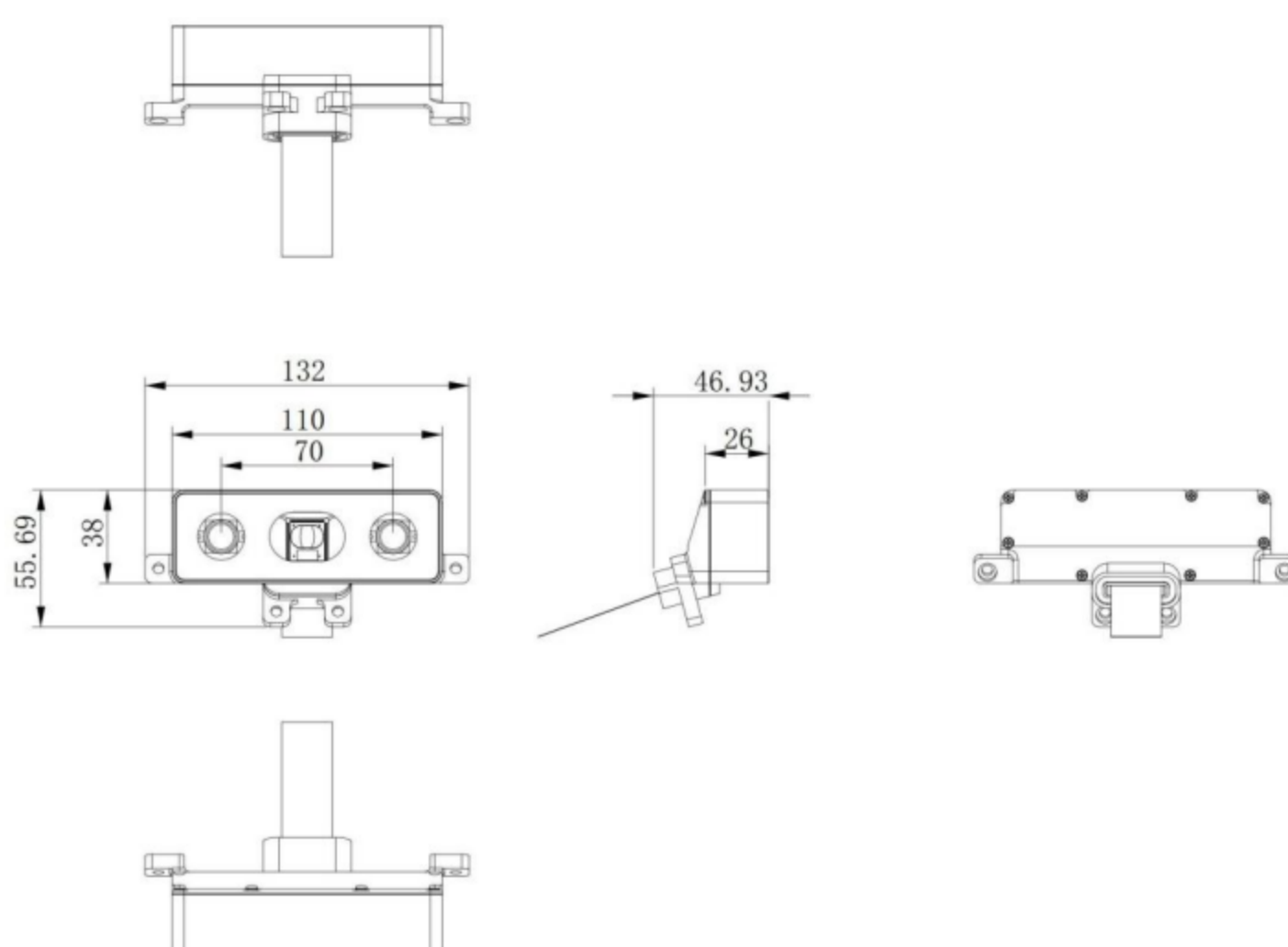
Module dimension drawing (132 × 55.69 × 46.93 mm)
